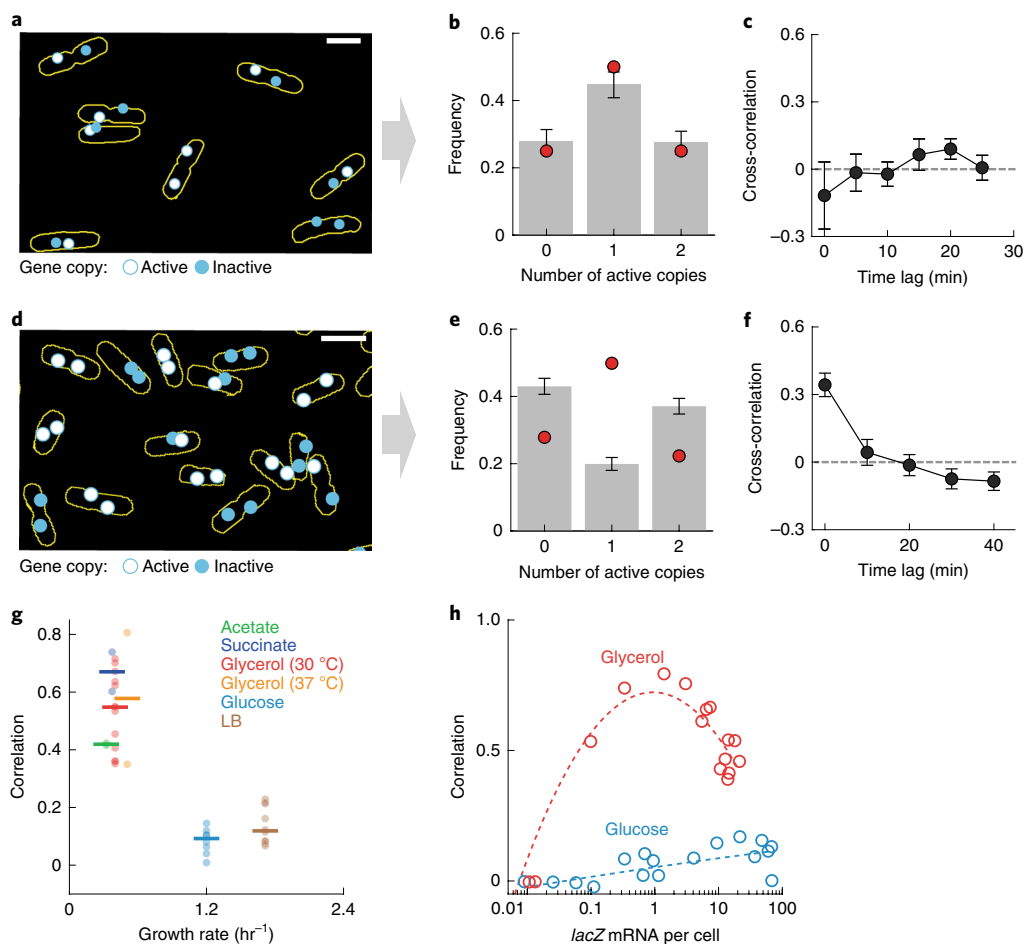
Fig. 3 | Promoter activity is coupled to the activity of additional gene copies in the cell. a , The transcriptional activity of individual copies of P_{lac} in cells grown in glucose (37 °C, 1 mM cAMP and 100 \mu M IPTG). For each cell that had two endogenous sister lac copies, the position and activity of each copy is overlaid on the cell boundary (yellow), as in Fig. 1b above ( lacZ mRNA is not shown). Scale bar, 2 \mu m. b , The distribution of the number of active P_{lac} copies in cells that had two copies of the gene. The grey bars show the data (normalized counts) for cells grown in glucose; error bars indicate the standard deviation. The red dots indicate the fit to a model assuming independent activity of the two copies (binomial distribution). c , The cross-correlation (mean \pm s.e.m.) between two copies of P_{lac} -48MS2bs in the same cell measured in live cells grown in glucose. d–f , The same as a–c , respectively, for cells grown in glycerol (30 °C, 10 \mu M IPTG). g , The correlation between sister copies of P_{lac} as a function of growth rate. The dots represent the data and the horizontal bars show the median across samples. Cells were grown in the following conditions: 30 °C in LB, 37 °C in glucose, 37 °C in glycerol, 30 °C in glycerol, 30 °C in succinate and 37 °C in acetate. h , The correlation between sister copies of P_{lac} as a function of expression level (total lacZ mRNA per cell) for cells grown in glucose and glycerol. The circles represent the data and the dashed lines are polynomial fits serving as a guide for the eye. See Supplementary Note for more details.
